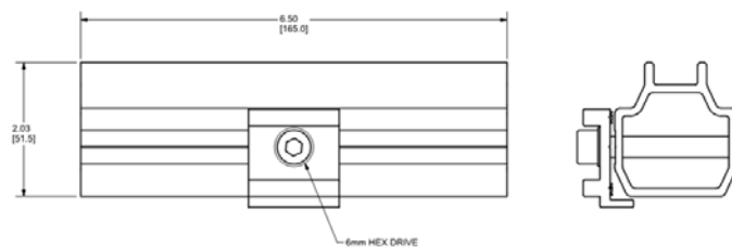
SMR200 Bonding Rail Splice
