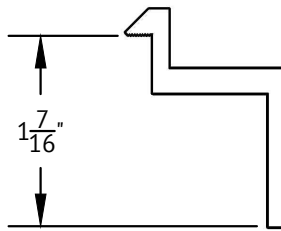
C CLAMP
