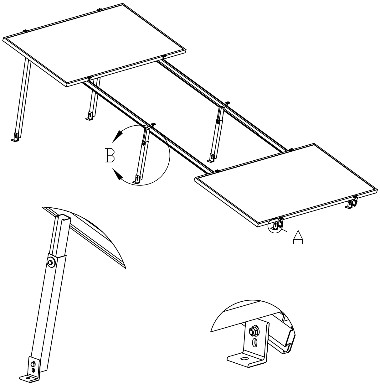
DETAIL A - L FOOT
