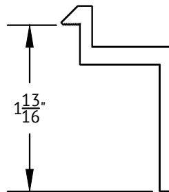
F CLAMP
