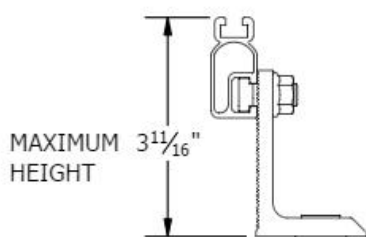
SOLARMOUNT LIGHT ON L-FOOT
