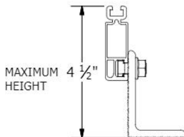
SOLARMOUNT STANDARD ON L-FOOT
