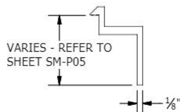
BONDING SM END CLAMP
