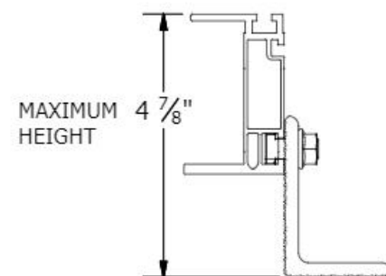
SOLARMOUNT HD ON L-FOOT
