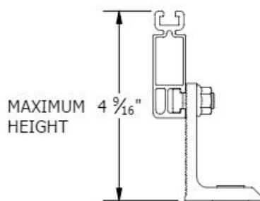
SOLARMOUNT STANDARD ON L-FOOT
